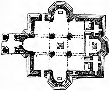
PLAN OF ETCHMIADZIN CATHEDRAL
