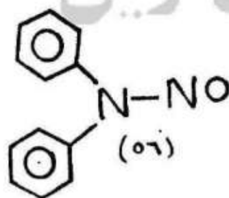
Diphenylnitrosamine
