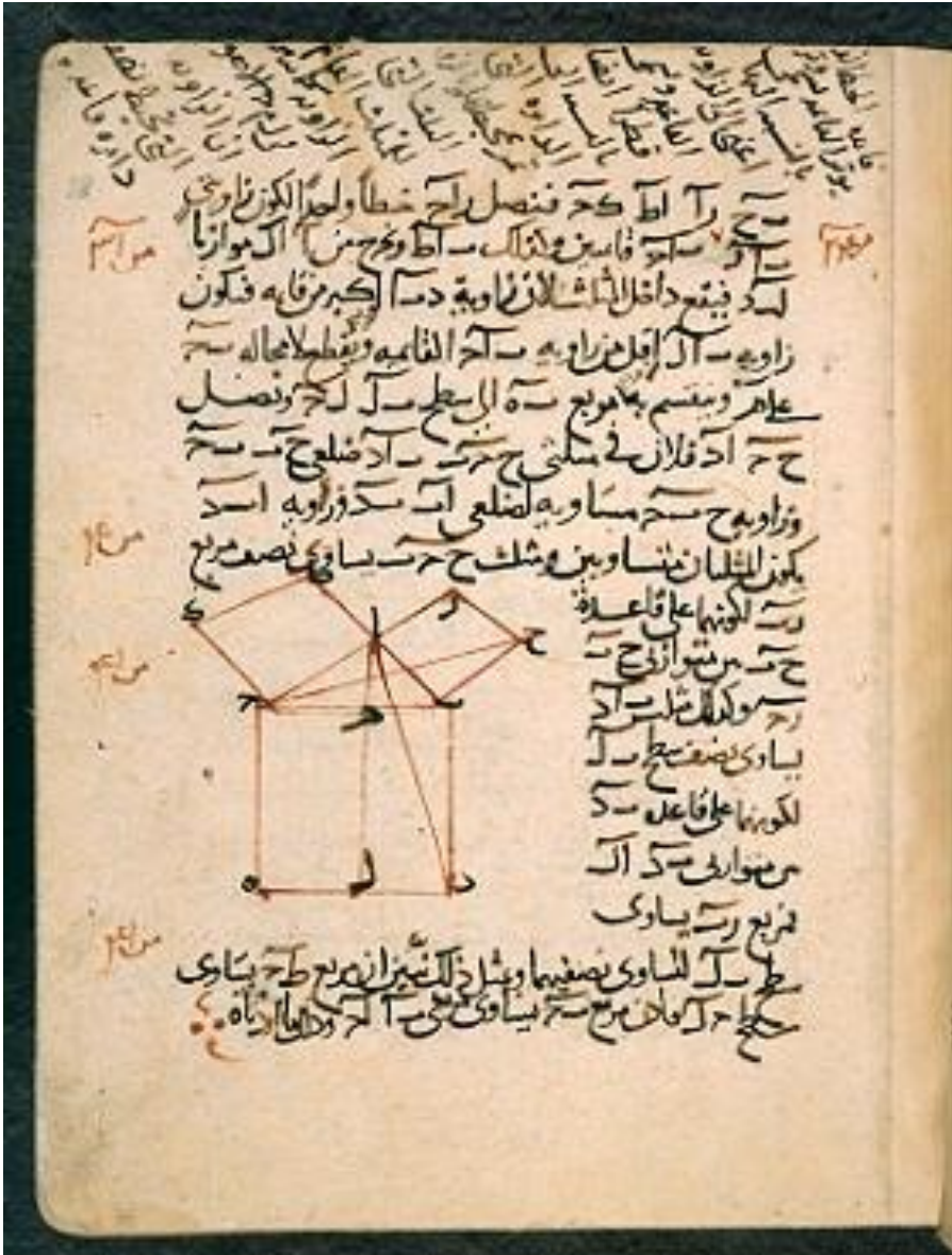
The Pythagorean theorem in the Arabic translation of Euclid's Elements. The manuscript copy is dated ۱۲۵۸.
